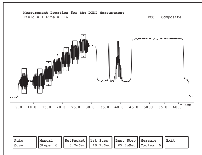
Measure Mode DGBP special position acquisition feature.
