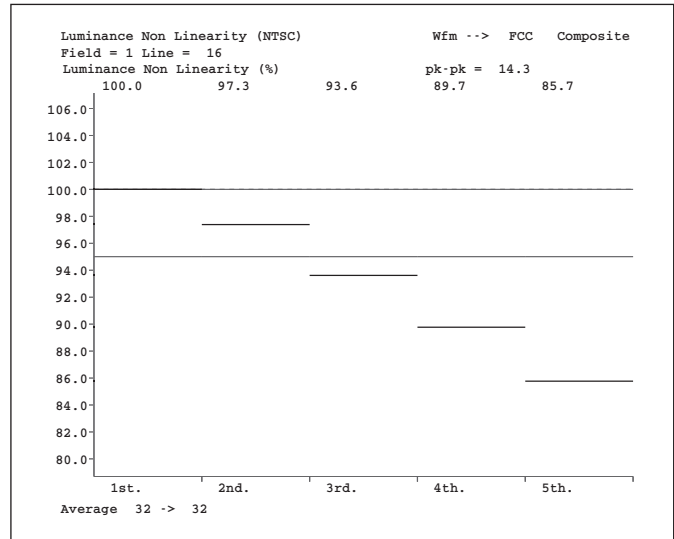
Luminance Non-Linearity measurement.
