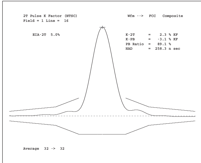
K-factor measurement.
