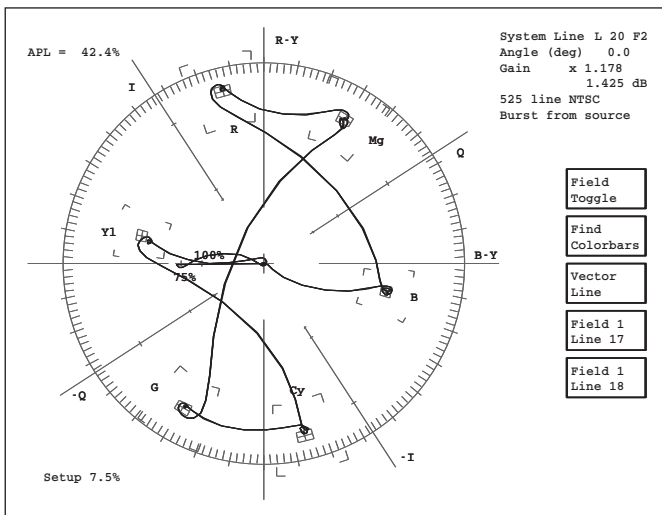
In Vector Mode, the VM700T becomes a digital vectorscope with an electronic graticule. A "Color Bar Search" feature makes it easy to quickly display a line containing a color bar test signal.
