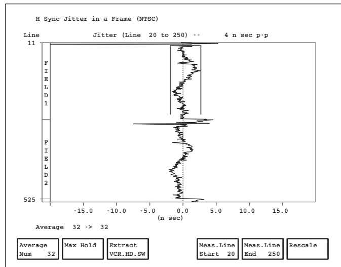
H_Jitter.
