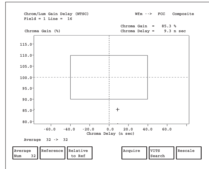
Chrominance to Luminance Gain and Delay measurement.
