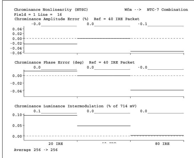
Chrominance Non-Linearity measurement.
