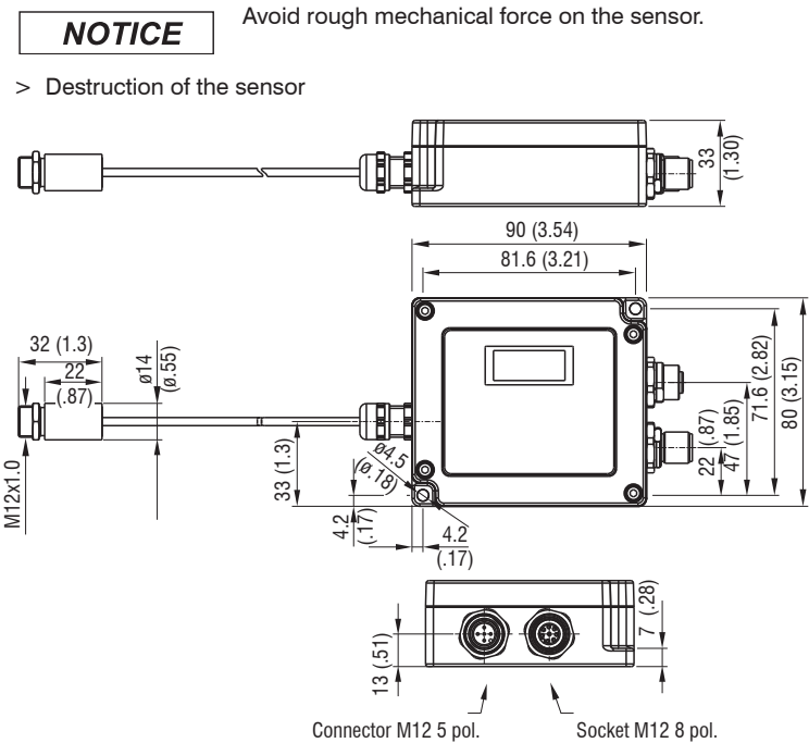
Dimensional drawing thermoMETER UC, dimensions in mm (inches, rounded off)
