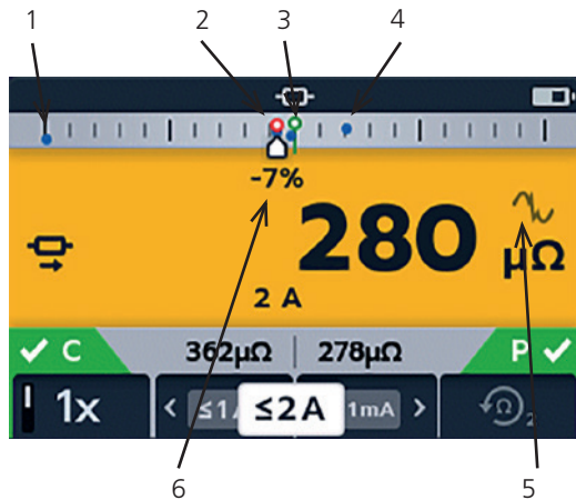
DLRO2 color display with new Difference Meter
