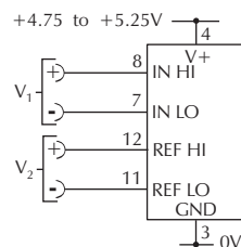
Check solder links 1 & 3 are OPEN.
