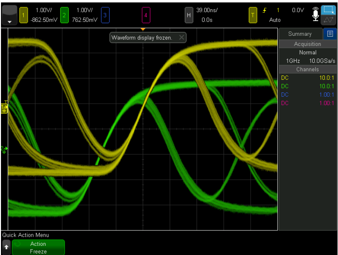
Figure 57. Quick Freeze Display preserves the persistence.
