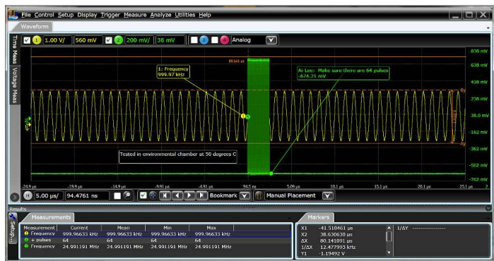
Figure 58. N8900A Infiniium Offline software.
