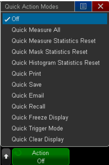
Figure 56. QuickAction menu.
