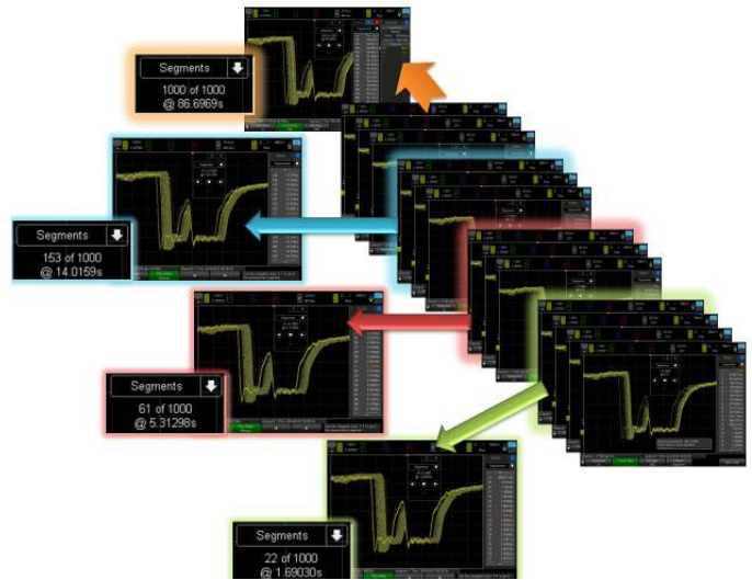
Figure 22. Segmented memory graphical representation.
