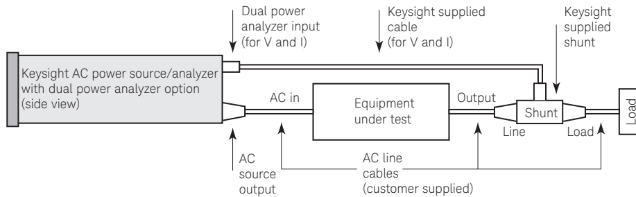
Figure 1. Test configuration of efficiency measurement using an Keysight AC source with the O20 dual power analyzer option.
