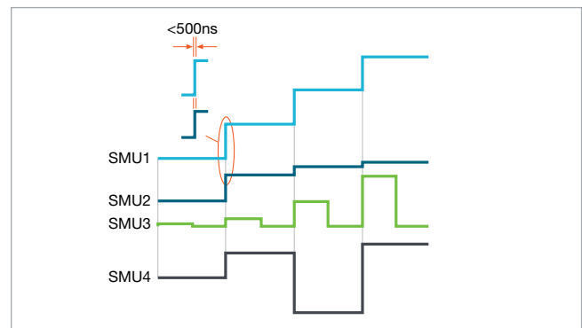
All channels in the TSP-Link system are synchronized to under 500ns.
