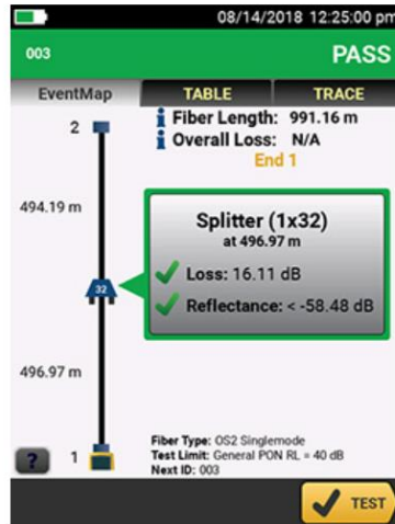
Splitter as seen on an EventMap
