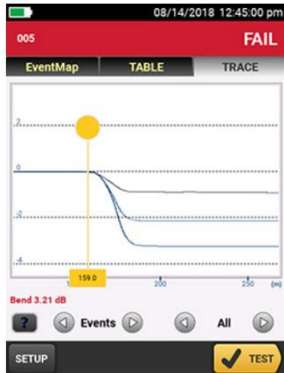
Bend as seen on an OTDR trace
