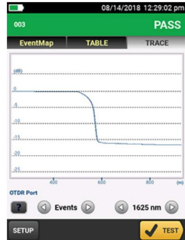
Splitter as seen on an OTDR trace
