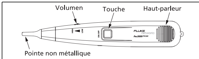
Figure 1. Sonde PRO3000
