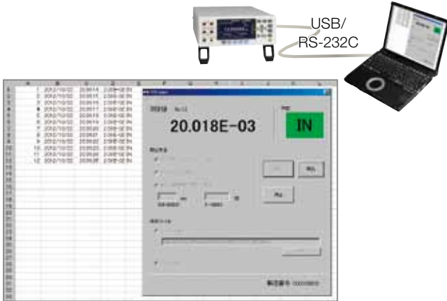
Applications screen
