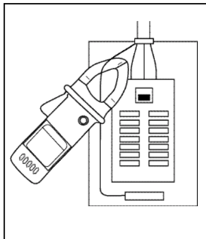
Figure 11: Measuring at the Service Entrance Panel
