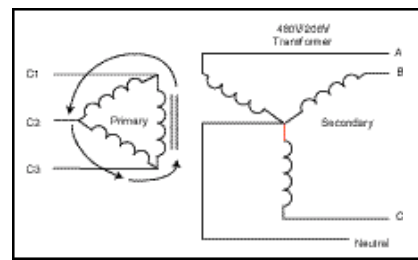
Figure 9: Delta Primary, Circulating Current
