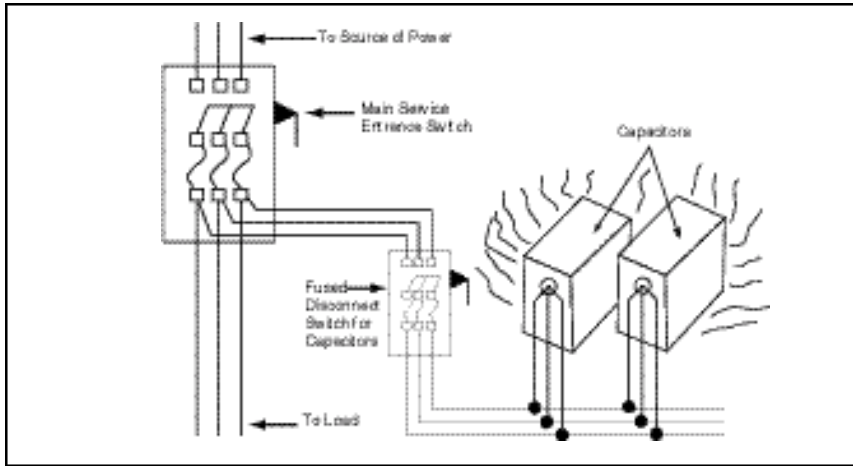
Figure 10: Power Factor Capacitors at Resonant Frequency
