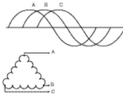
Figure 2: 3Ø, 3-Wire System
