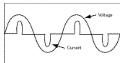
Figure 7: Nonlinear Current Draw
