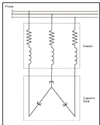
Figure 13: Single tuned shunt filter
