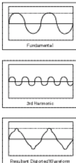
Figure 6: Composite Waveform
