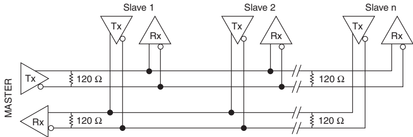
Figure 11. 4-Wire Full-Duplex Multidrop Network Using Terminating Resistors
