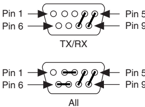
Figure 8. RS-485/422 Loopback
