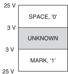
Figure 7. RS-232 Signals
