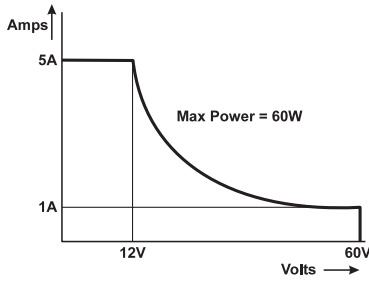
Autoranging Curve for 60 V/5 A/60 W Power Module
