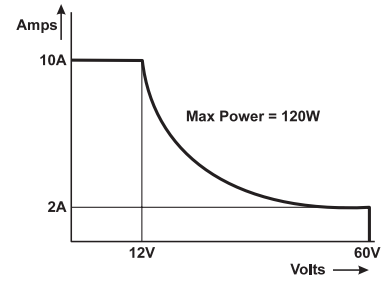
Autoranging Curve for 60 V/10 A/120 W Power Module
