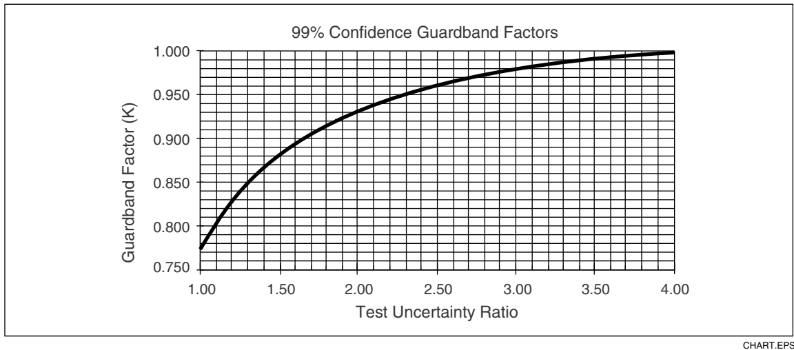
Figure 3-18. Determining Other Test Limits
