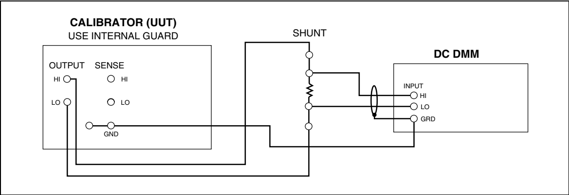
Figure 3-7. Direct Current Accuracy Test Setup
