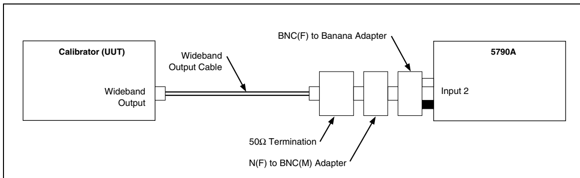
Figure 3-14. Wideband Accuracy at 1 kHz Test Setup
