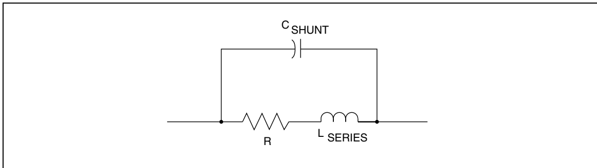
Figure 3-12. Metal Film Resistor Equivalent Circuit
