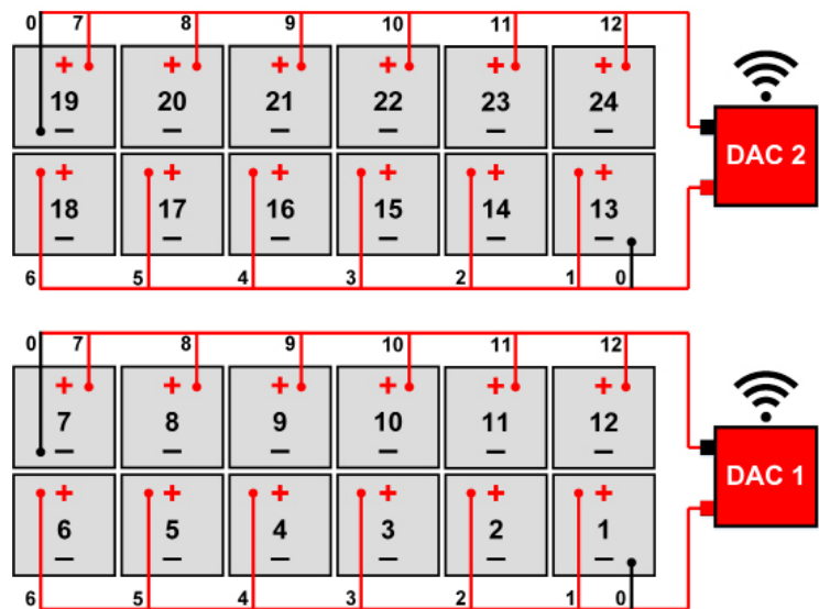
DAC Connection to 48V System (2V Cells)
