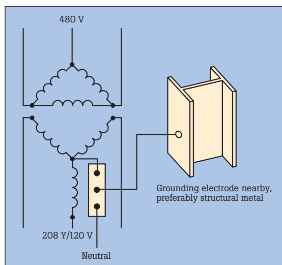
Figure 3. Transformer grounding.
