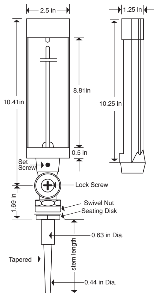
Dimensions for 9" Case Models
