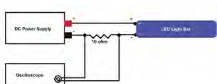
Example LED test setup
