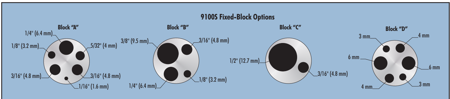
9100S fixed-block options. Order number 9100S-A, 9100S-B, 9100S-C or 9100S-D for the desired block option.
