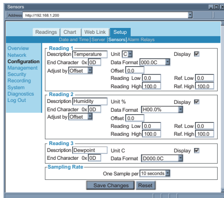
iTHX Sensor Configuration
