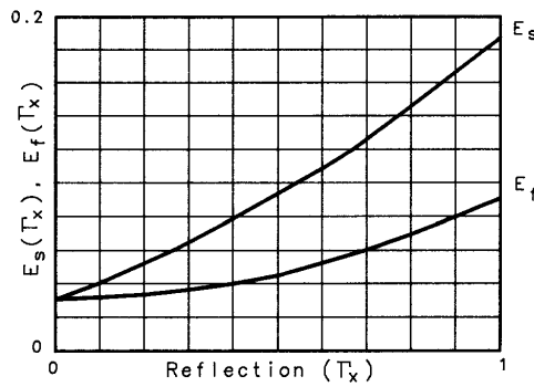
Figure 5 772D Error 2.0 to 12.4 GHz
