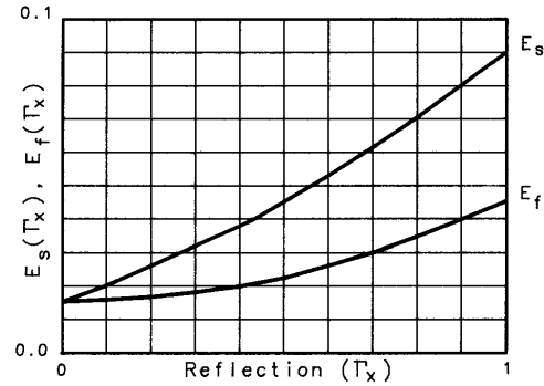
Figure 4 772D Error 0.1 to 2.0 GHz
