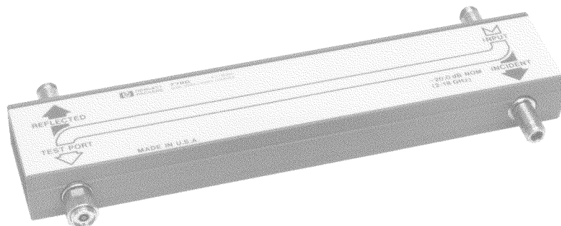
Figure 7 772D Dual Direction Coupler
