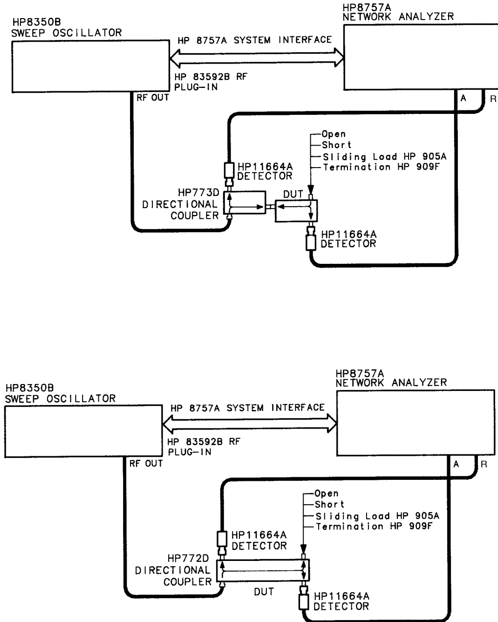
Figure 9 772D/773D Performance Test Setup
