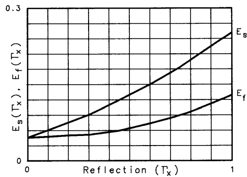
Figure 6 772D Error 12.4 to 18.0 GHz
