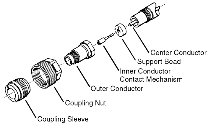
Figure 10 Use and Care of APC-7 Connectors
